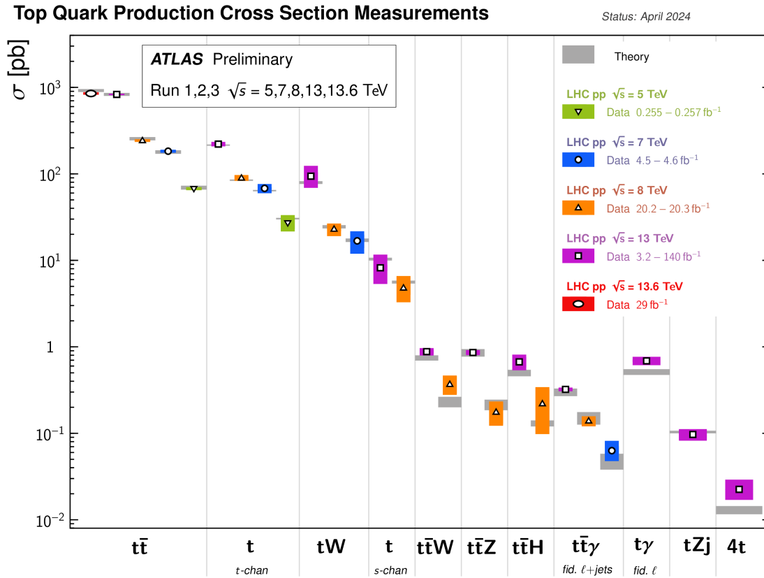
Figure 2.2.: Summary of several t quark related production cross-section measurements. The theoretical expectations were calculated at next to leading order or higher [48].
