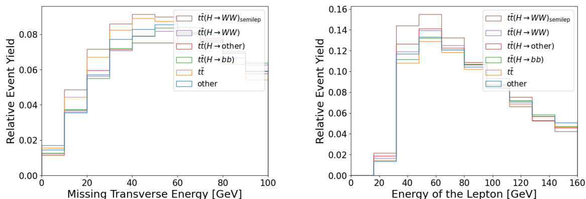
Figure 7.2.: Distributions of different event topologies for (left) the missing energy per event and (right) the energy of the identified lepton.
