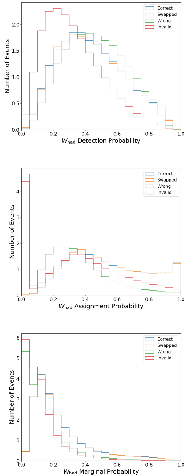
Figure A.3.: Normalised distributions of SPA-Net 's output probabilities for the hadronic W -boson from the H -boson decay.
