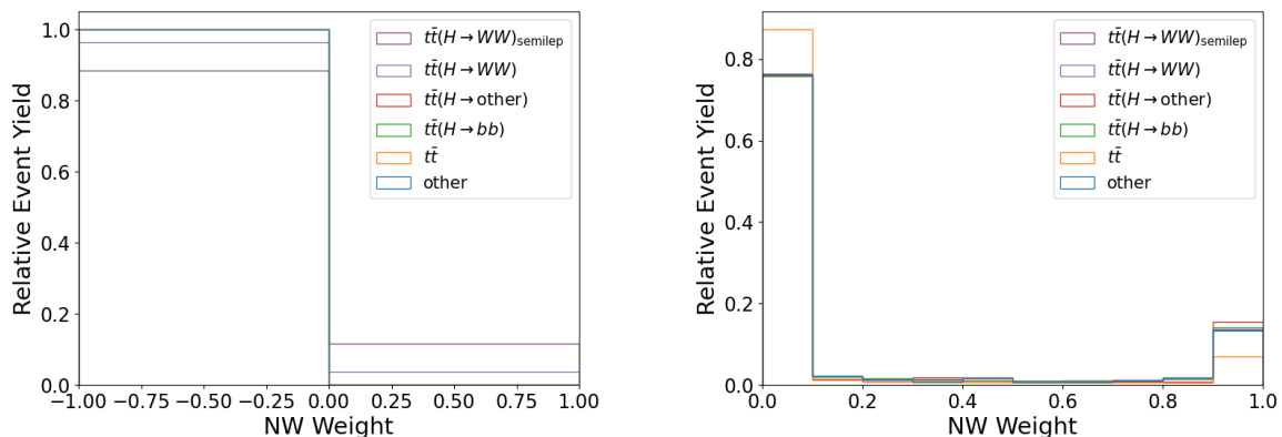
Figure 7.4.: Distributions of different event topologies for Neutrino Weighting output weight while (left) including events without any solution and (right) excluding events without any solution. Events with no solution are visualised as negative weight.
