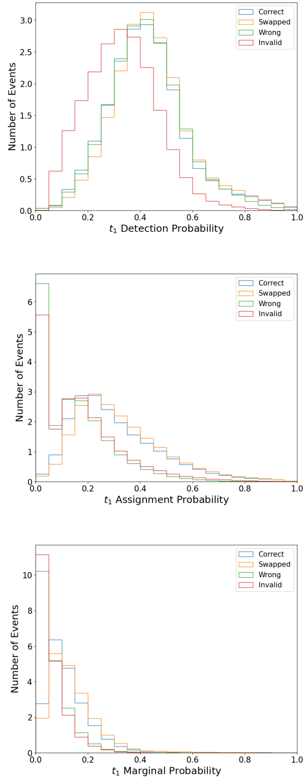
Figure A.1.: Normalised distributions of SPA-Net 's output probabilities for the t_1 quark.
