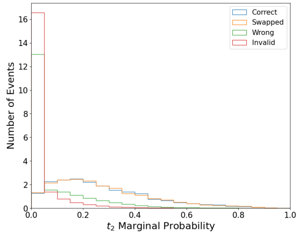
Figure A.2.: Normalised distributions of SPA-Net 's output probabilities for the t_2 quark.
